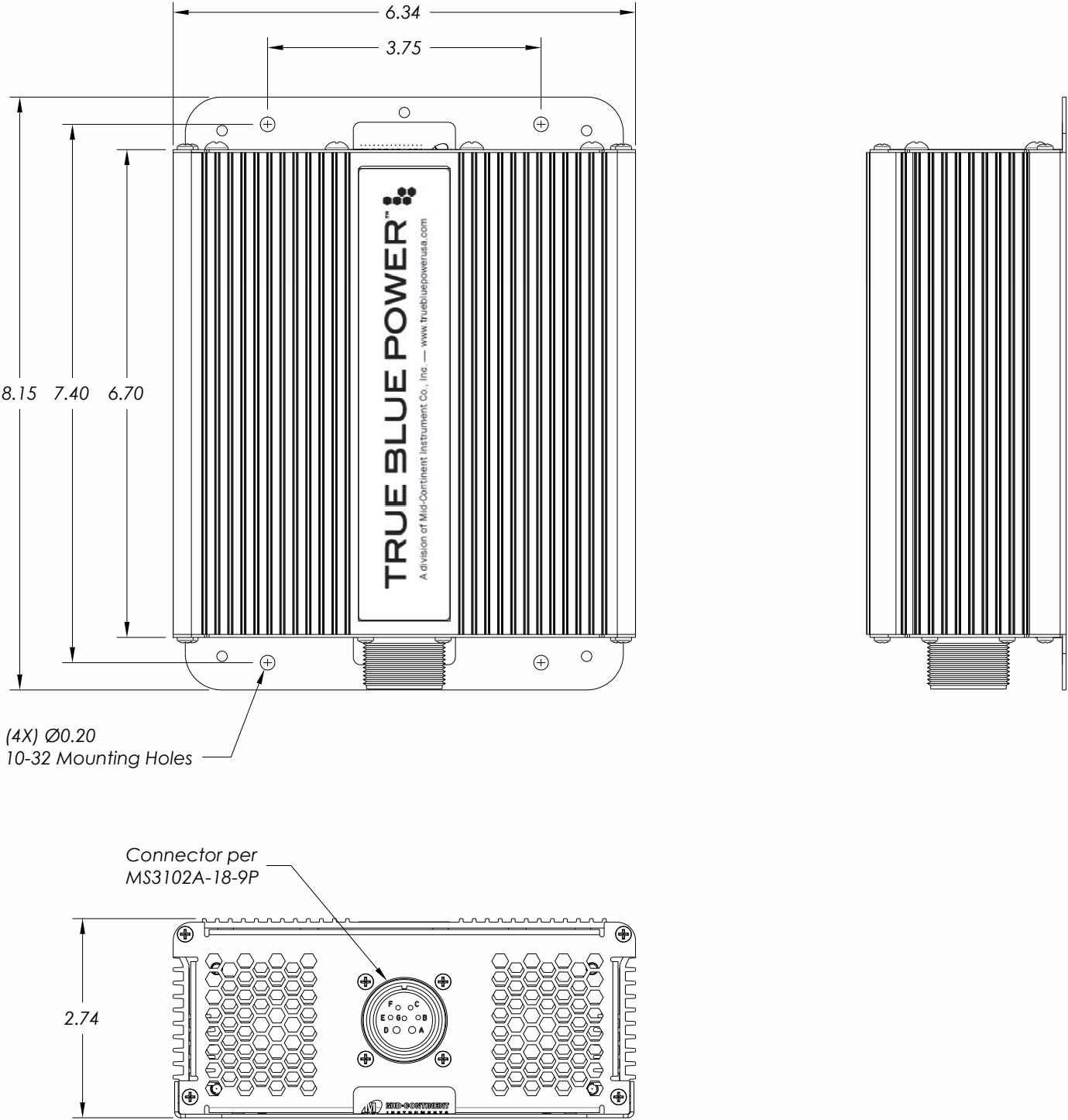
FIGURE 3.5 TI500 OUTLINE DRAWING
